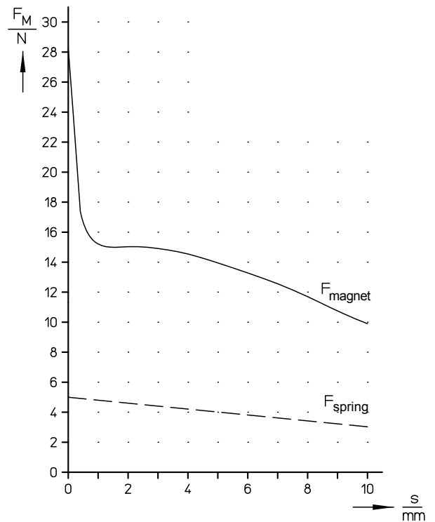
Fig. 15: Magnetic force-stroke-characteristic and return spring
