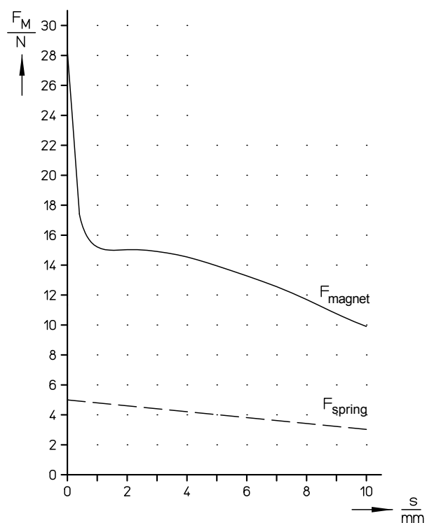
Fig. 12: Magnetic force-stroke-characteristic and return spring
