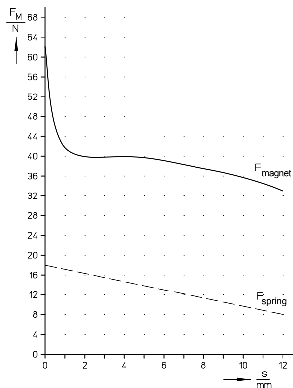
Fig. 19: Magnetic force-stroke-characteristic and return spring
