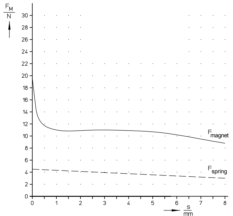
Fig. 4: Magnetic force-stroke-characteristic and return spring
