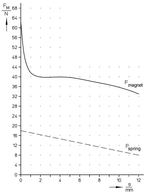
Fig. 22: Magnetic force-stroke-characteristic and return spring
