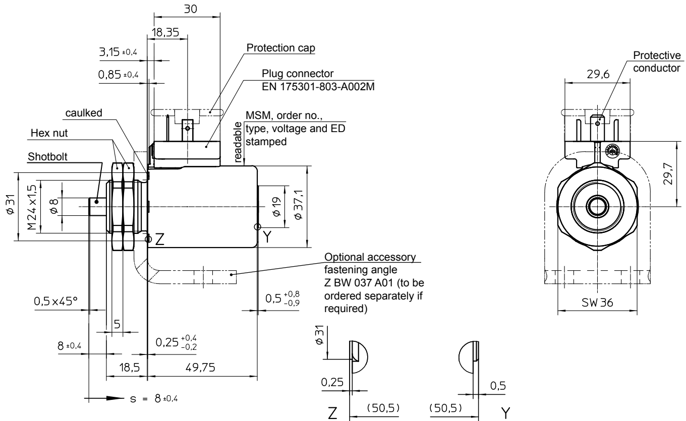
Fig. 2: Description in de-energised condition
