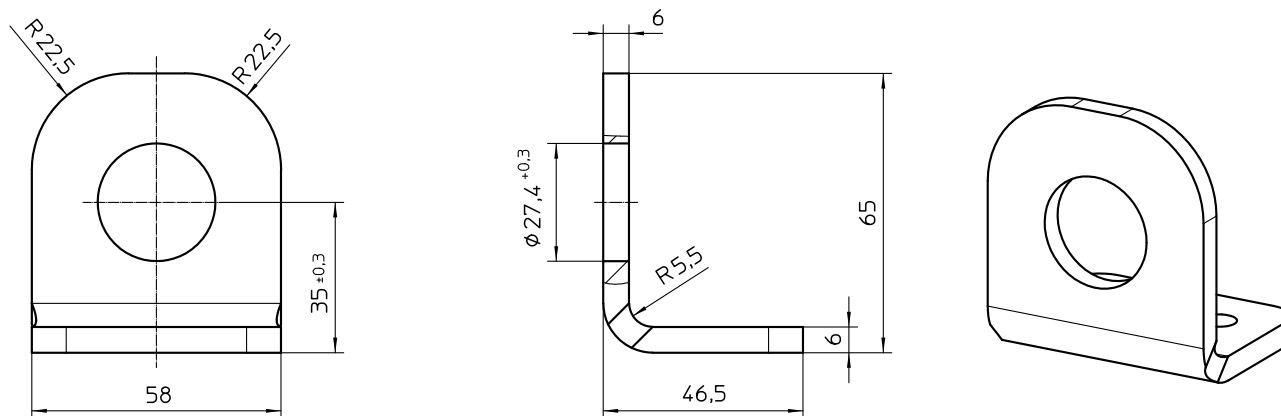
Fig. 25: Fastening angle Z BW 037 A01
