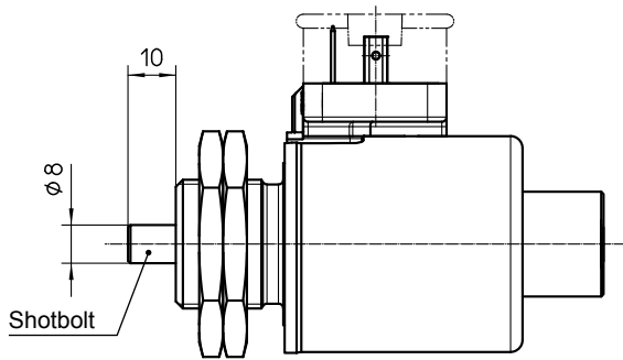
Fig. 14: Description in energised condition
