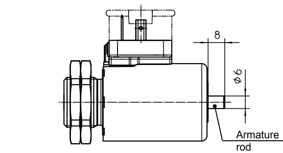
Fig. 3: Description in energised condition
