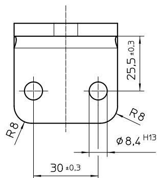
Fig. 25: Fastening angle Z BW 037 A01
