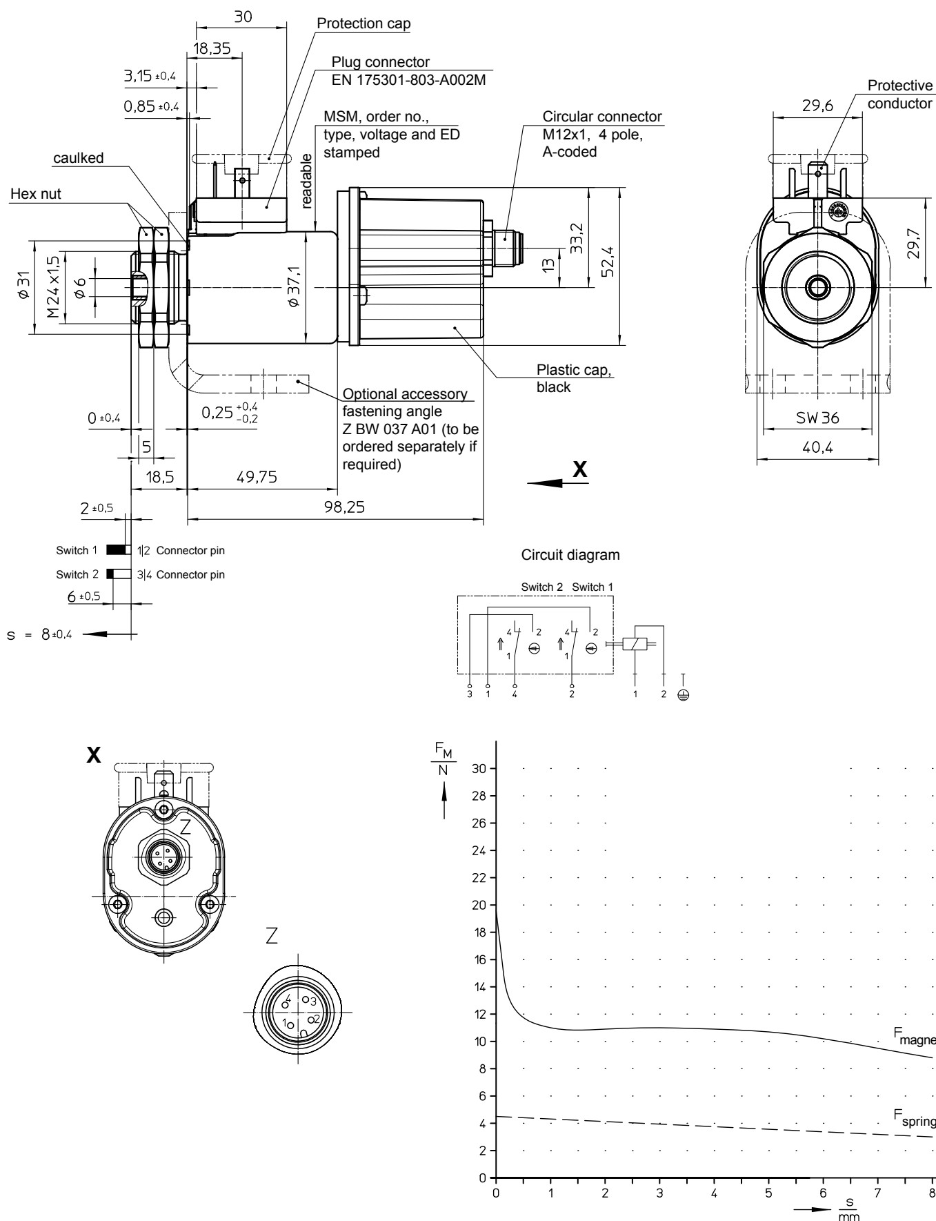
Fig. 9: Magnetic force-stroke-characteristic and return spring
