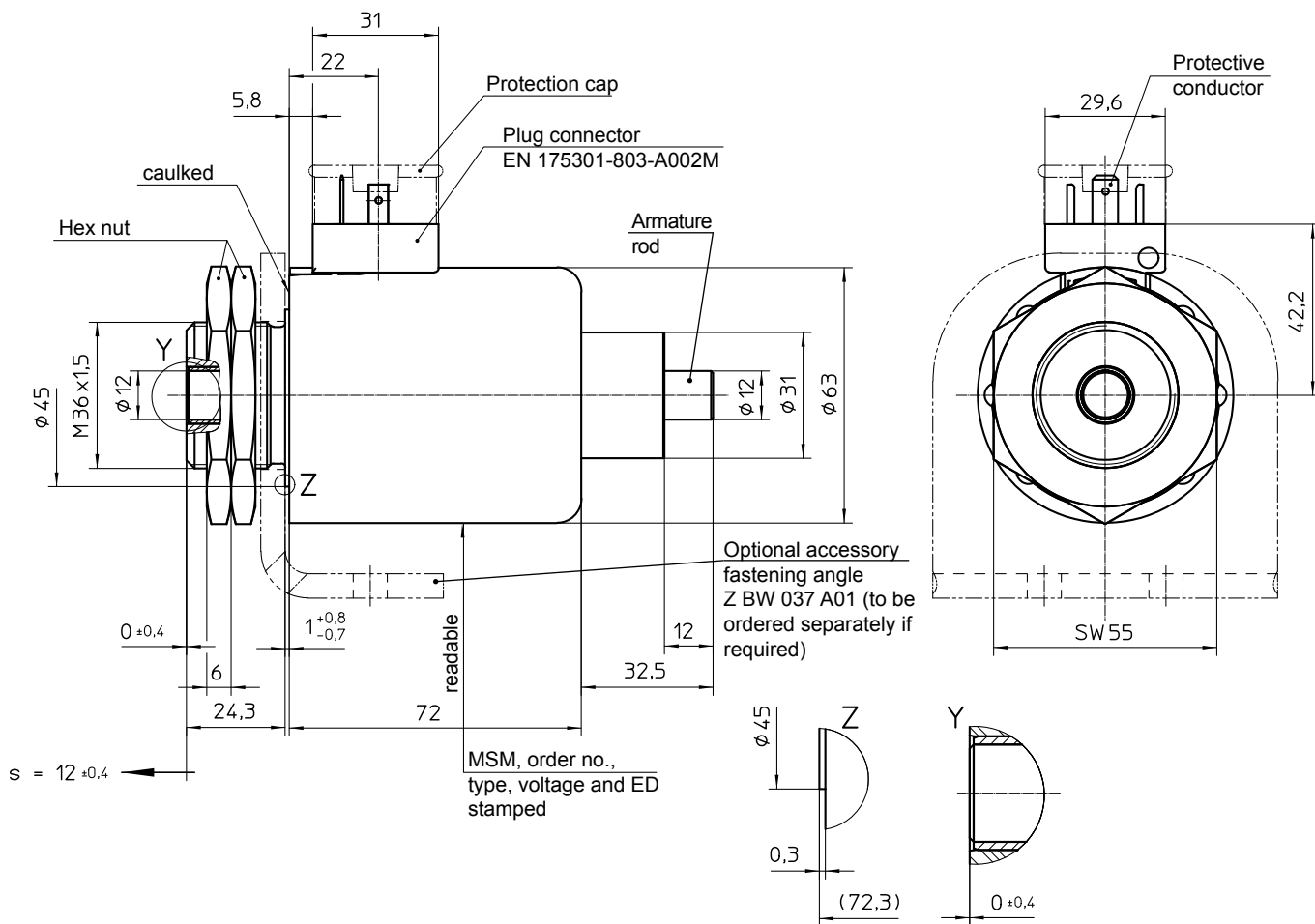
Fig. 20: Description in de-energised condition
