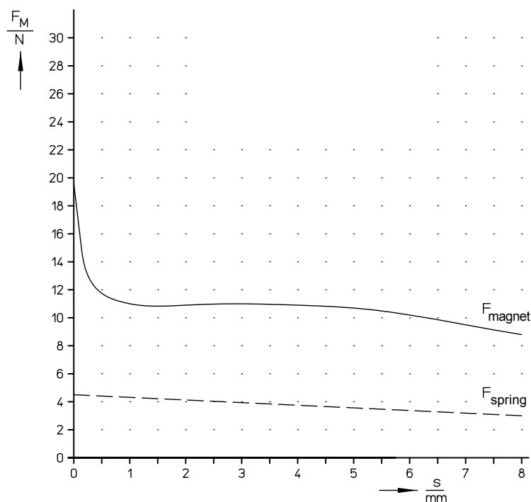
Fig. 7: Magnetic force-stroke-characteristic and return spring
