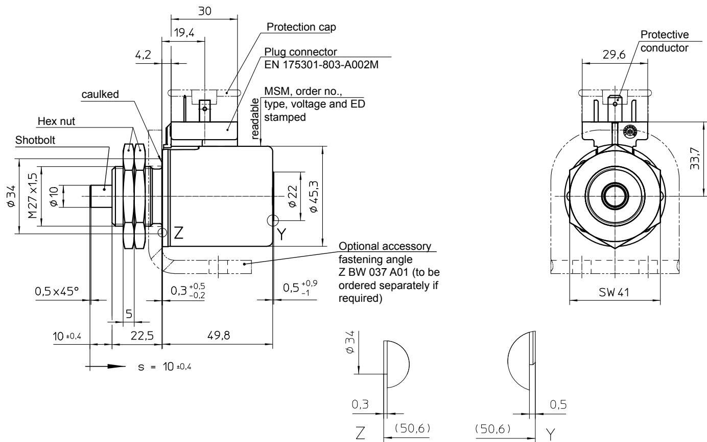
Fig. 10: Description in de-energised condition
