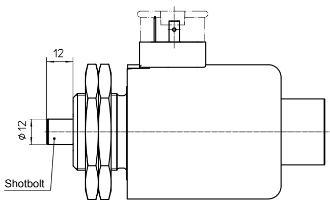
Fig. 21: Description in energised condition
