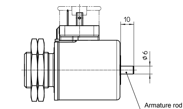
Fig. 11: Description in energised condition
