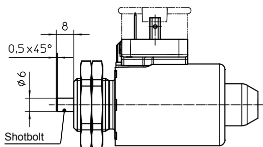
Fig. 6: Description in energised condition
