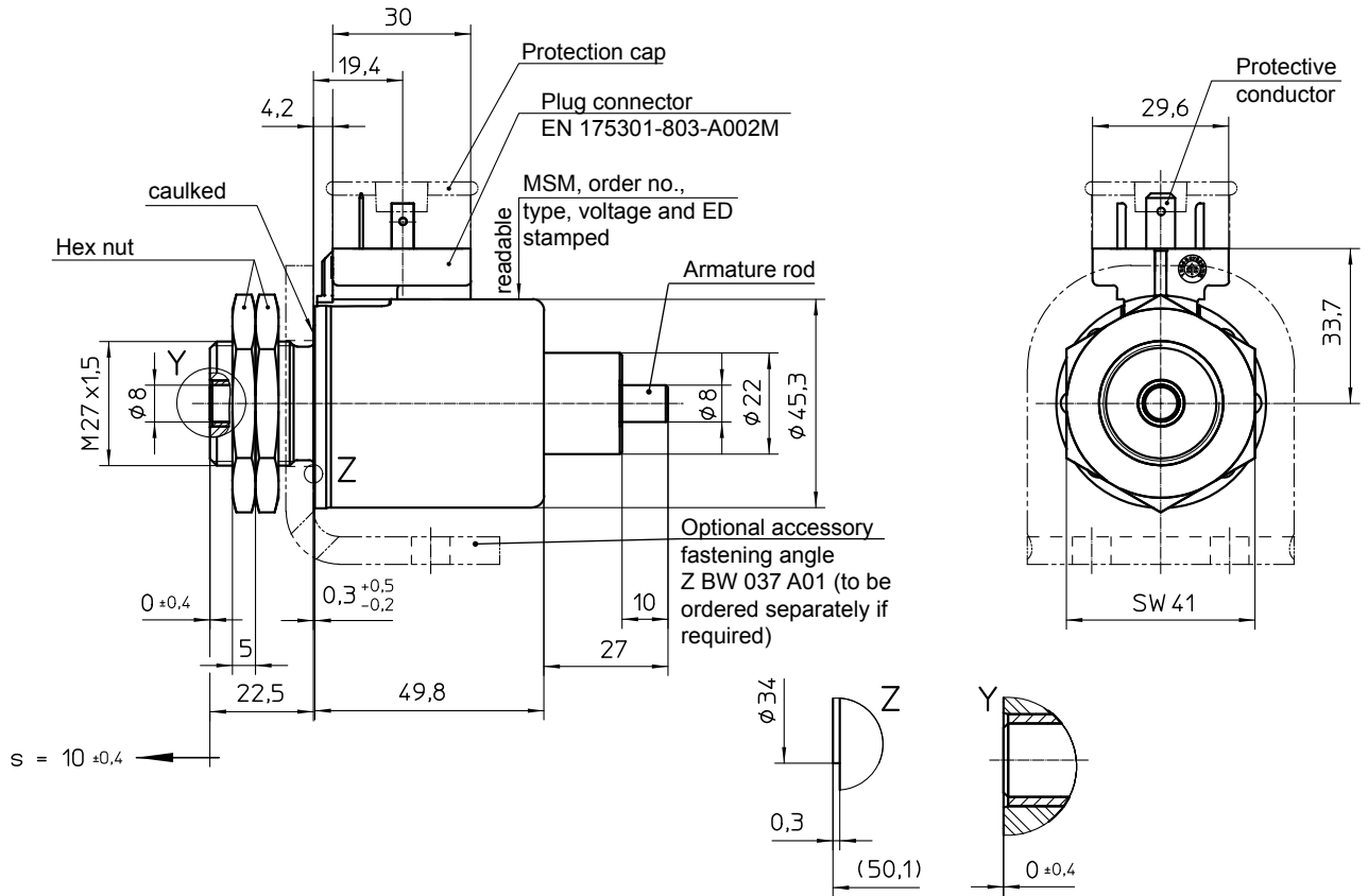
Fig. 13: Description in de-energised condition
